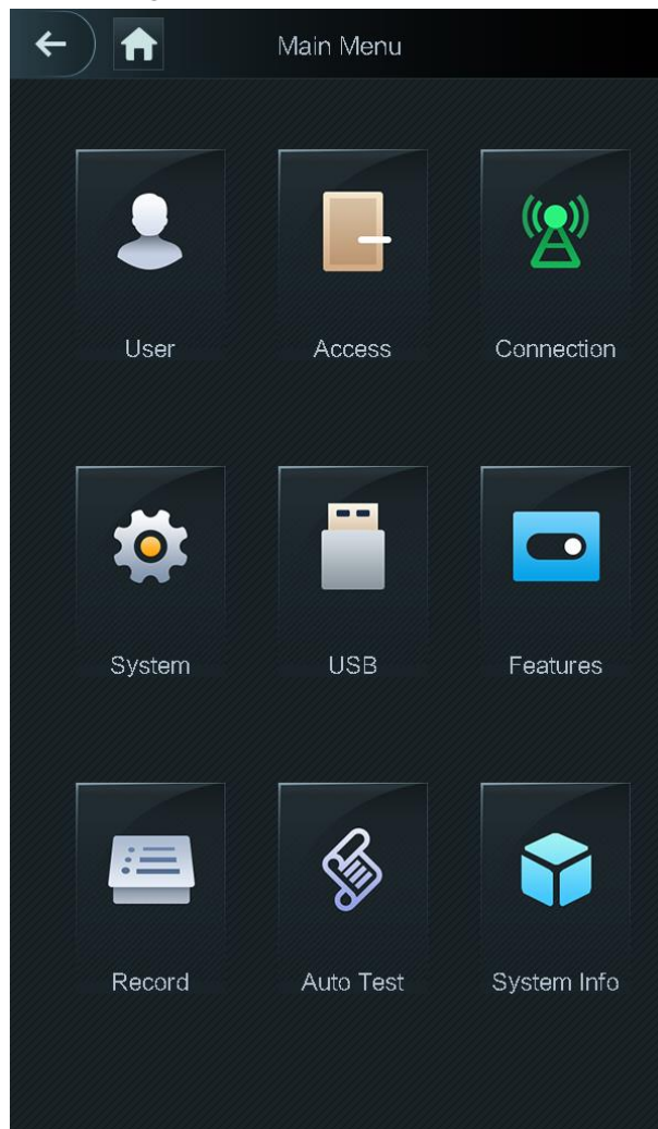
Figure 1-12 Main menu
