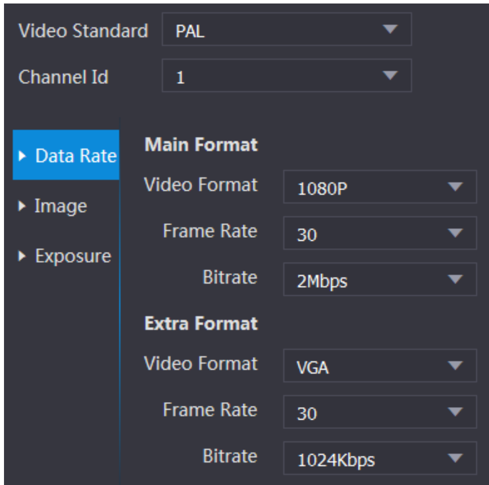
Figure 1-44 Data rate
