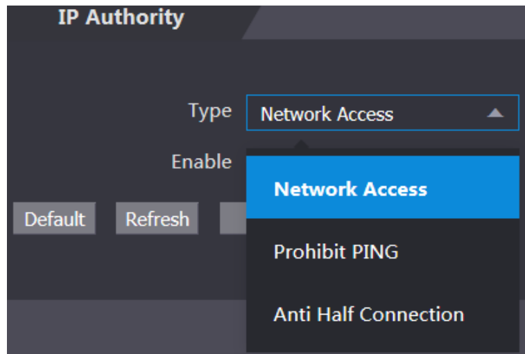
Figure 1-54 IP authority
