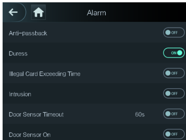
Figure 1-18 Alarm
