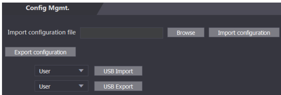
Figure 1-59 Configuration management
