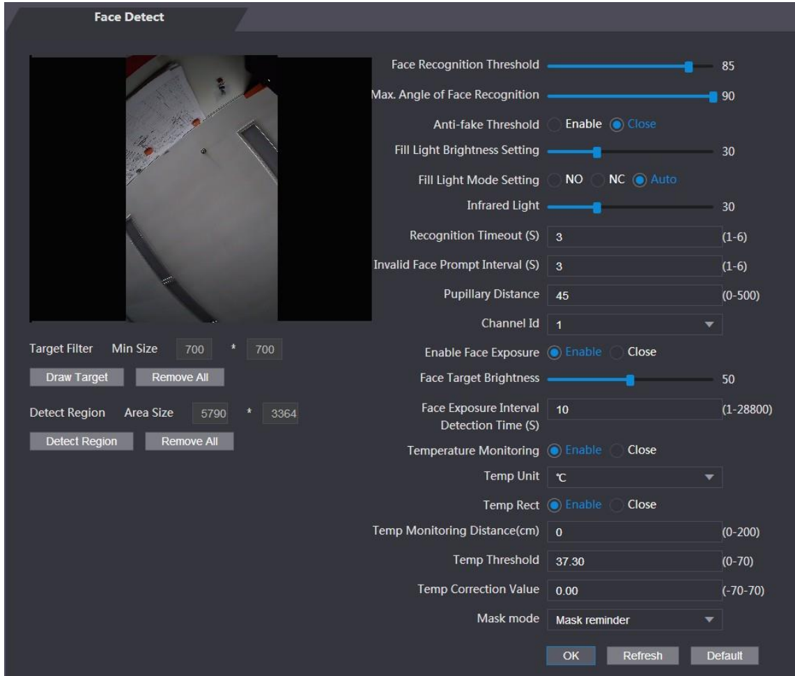
Figure 1-50 Face detect
