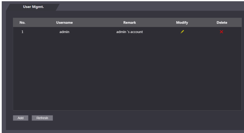
Figure 1-56 User management
