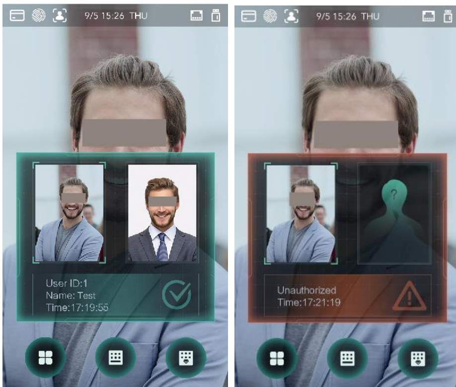
Figure 1-27 Mode 1
