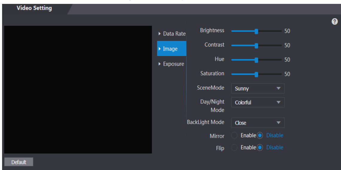
Figure 1-45 Image
