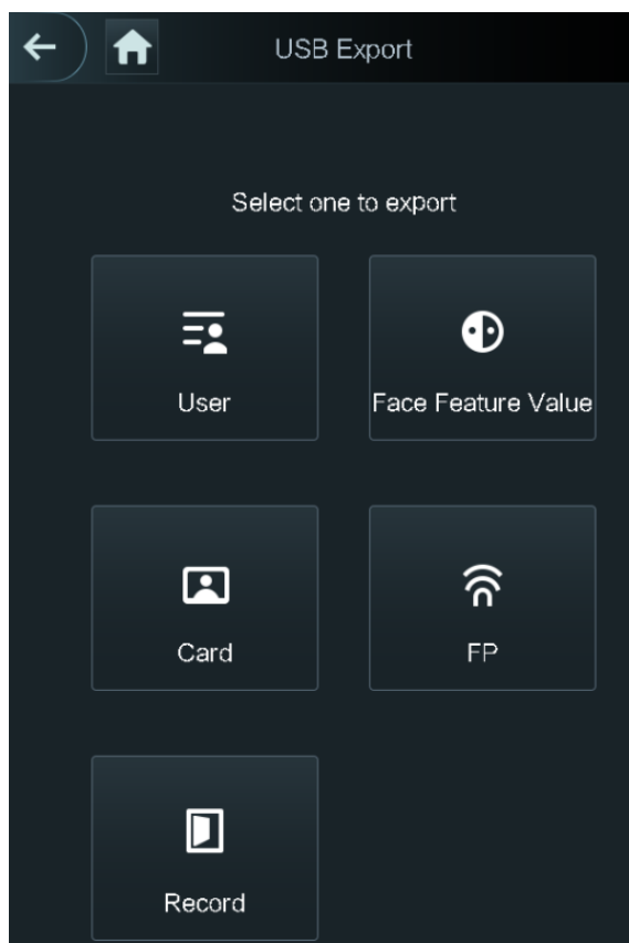
Figure 1-23 USB export
