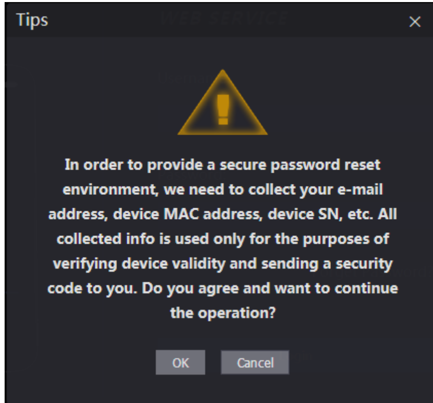
Figure 1-37 Tips
