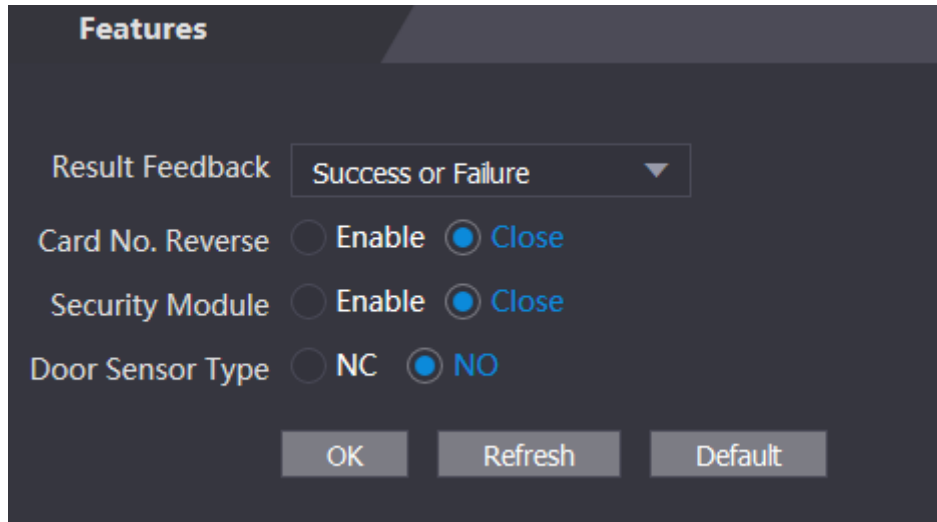
Figure 1-60 Features
