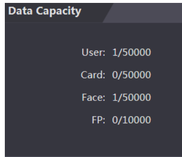
Figure 1-43 Data capacity
