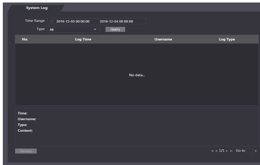
Figure 1-64 System log
