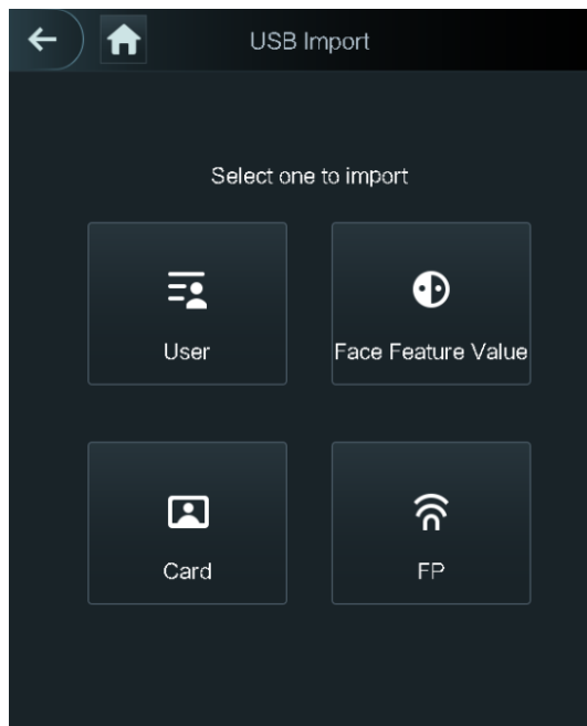
Figure 1-24 USB Import
