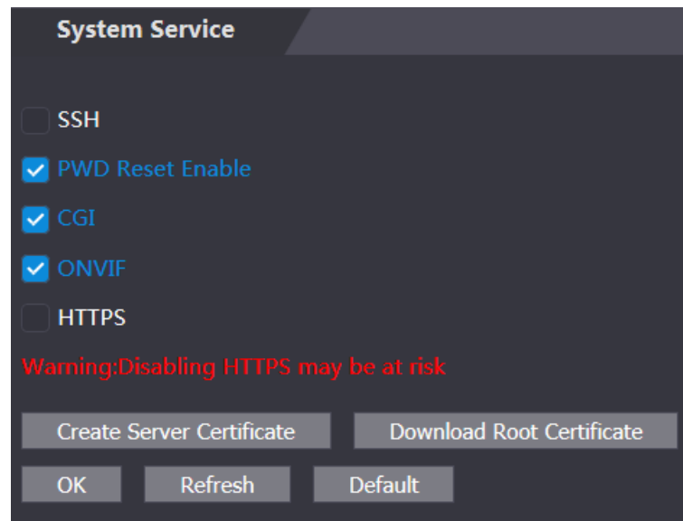
Figure 1-55 System service
