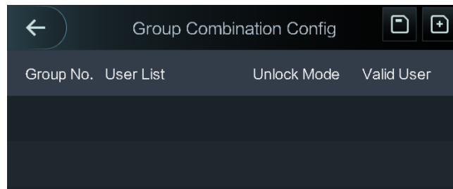
Figure 1-16 Group Combination
