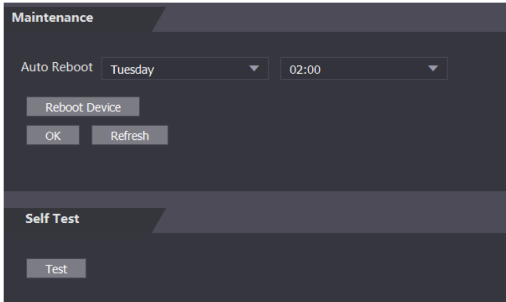
Figure 1-58 Maintenance
