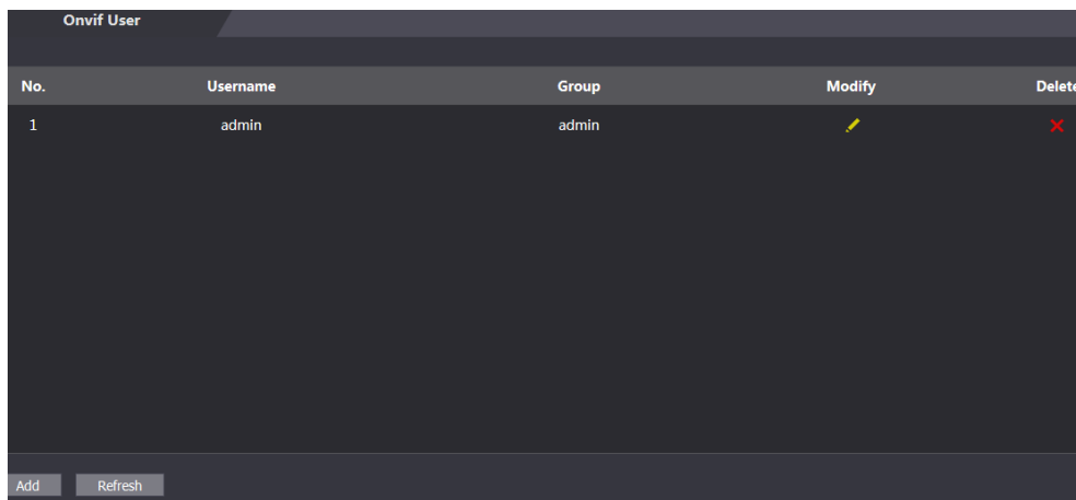
Figure 1-57 Onvif user
