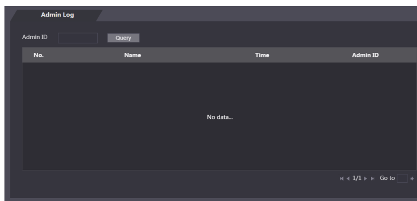
Figure 1-65 Admin log
