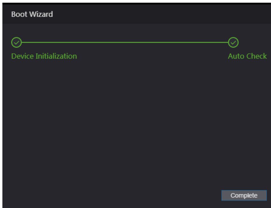
Figure 1-35 Finished configuration
