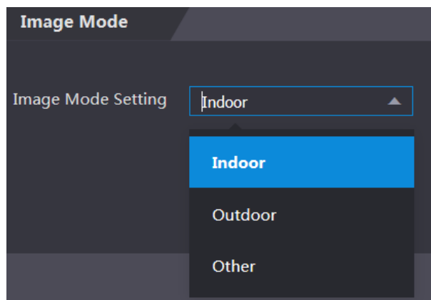
Figure 1-49 Image mode
