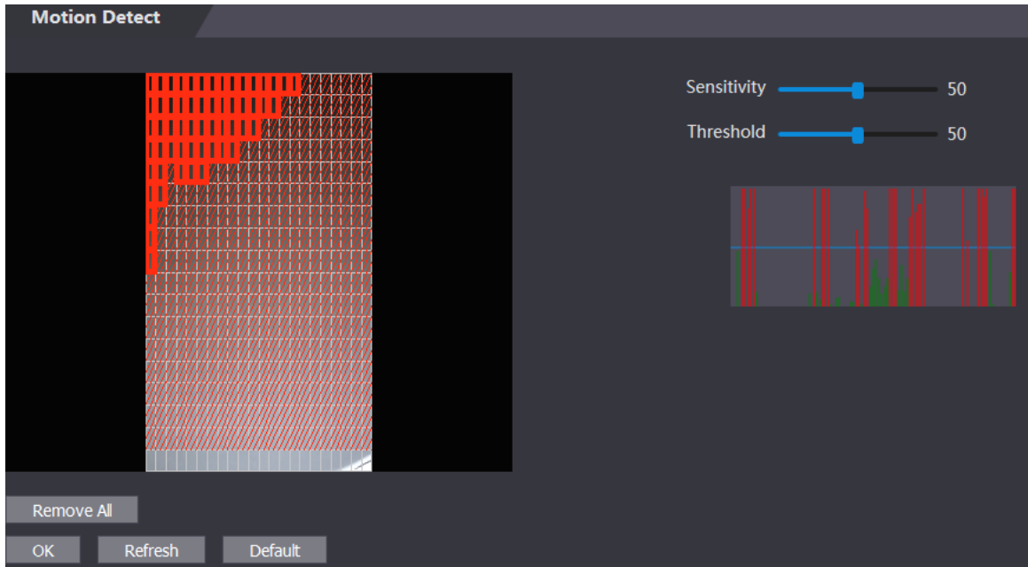
Figure 1-46 Motion detection
