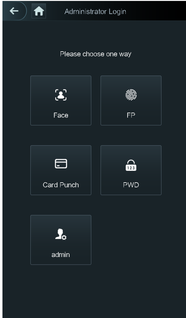
Figure 1-11 Administrator login
