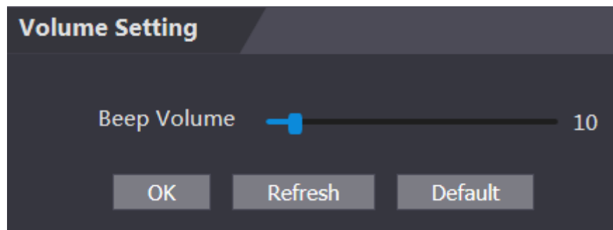
Figure 1-48 Volume setting
