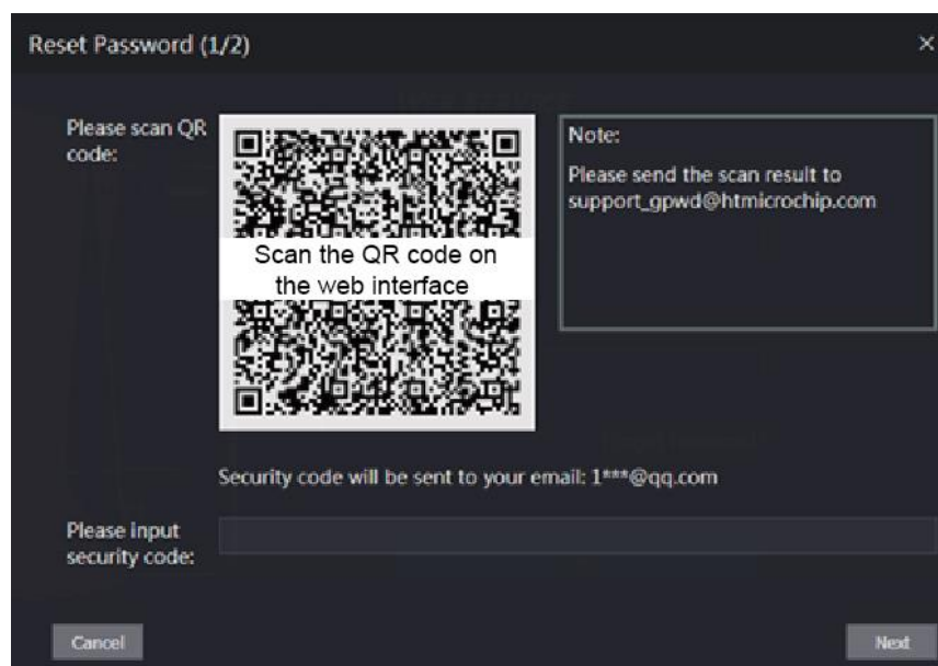
Figure 1-38 Reset Password
