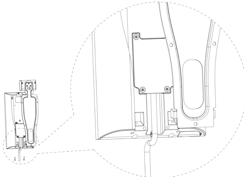
Figure 1-7 Applying silicon sealant
