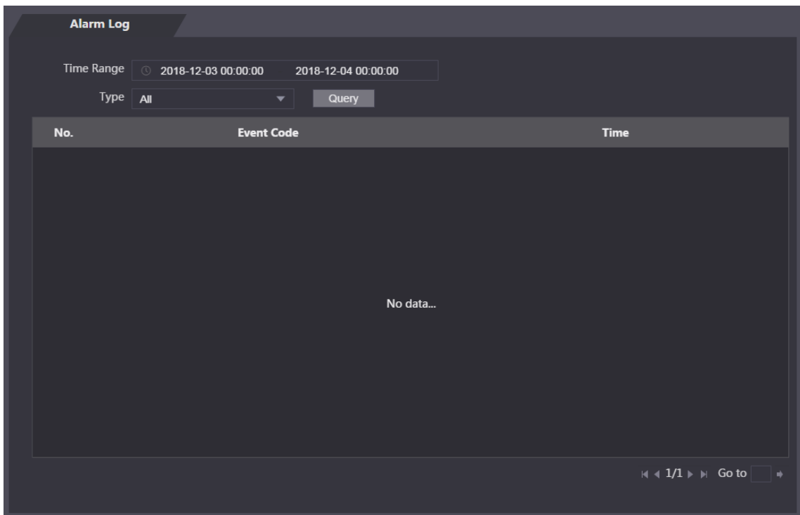
Figure 1-41 Alarm log
