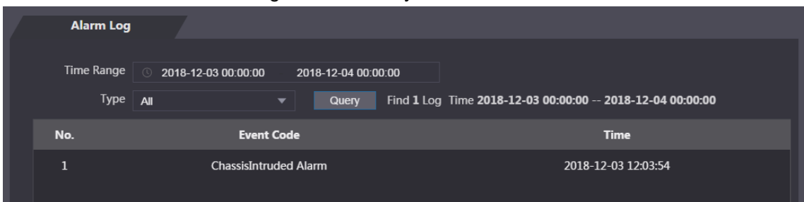
Figure 1-42 Query results
