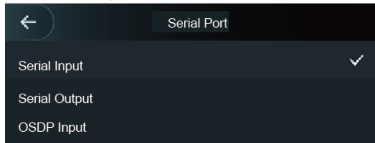
Figure 1-20 Serial port
