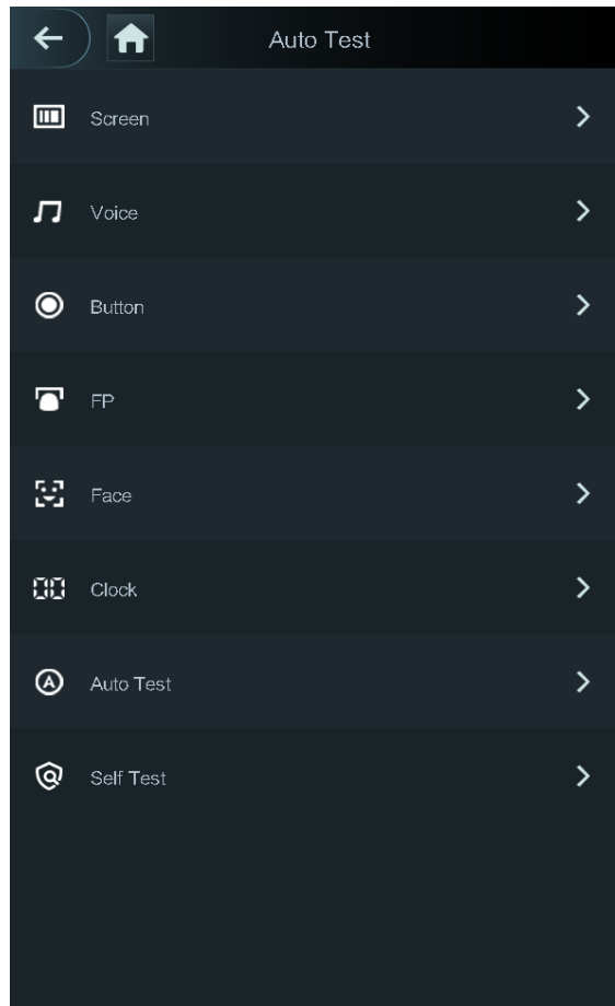
Figure 1-32 Auto test
